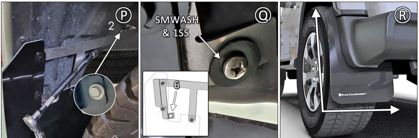
FIGURE R Ensure flap is parallel to even ground before tightening washers just until flush against flap.
