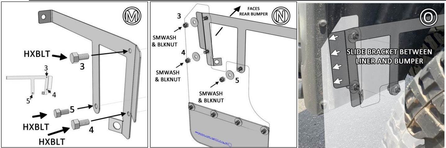
FIGURE P Use factory fastener 2 to secure bracket mount 2.
